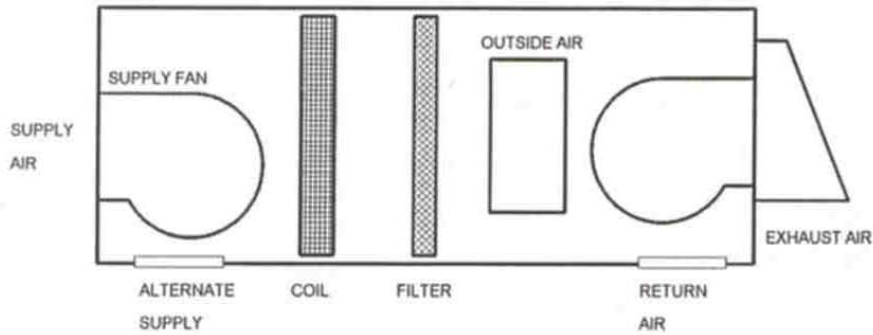
Economizer with Exhaust Fan
