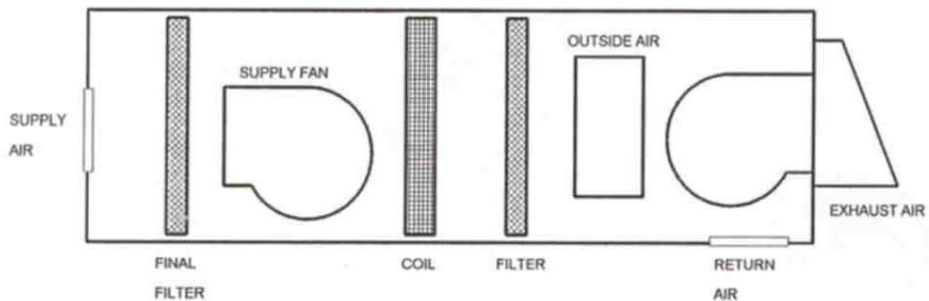
Economizer with Exhaust Fan and Final Filter
