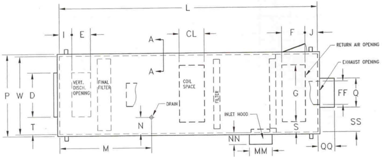
PLAN VIEW
